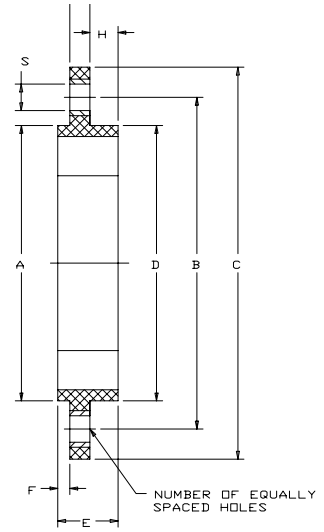
Universal Element
