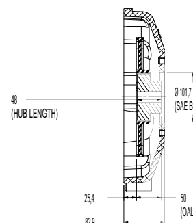
Ford VSG 413 - Shown with LK 100
