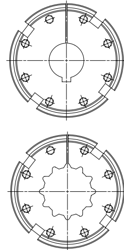
Shaft Lock
