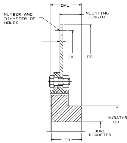
2-Piece Flange
