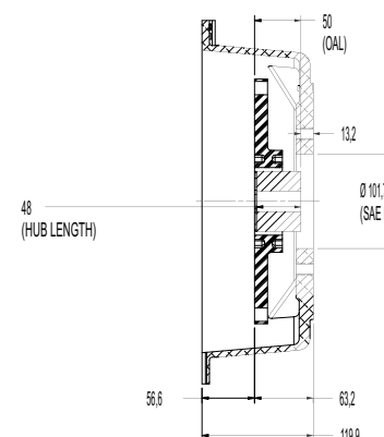
Perkins® 104-22 - Shown with LK 100
