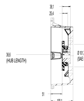
Kubota Super 05 - Shown with LK 80
