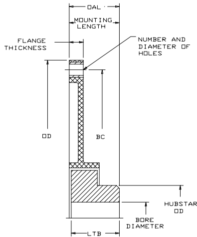
1-Piece Flange
