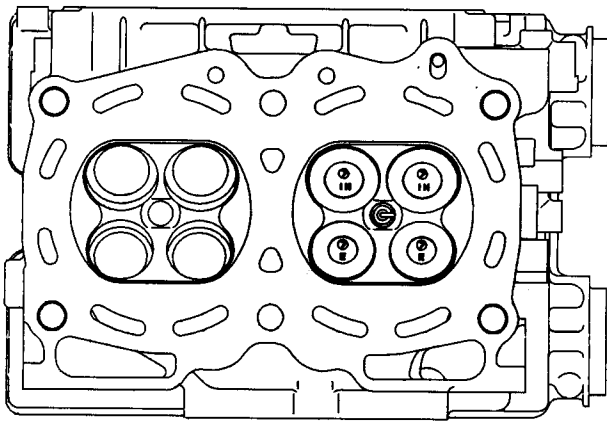
Fig. 15 DOHC 4 valve cylinder head
