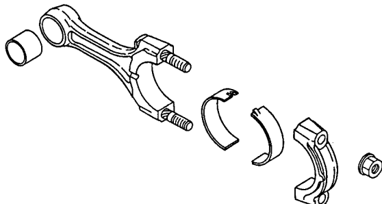
Fig. 8 Connecting rod
