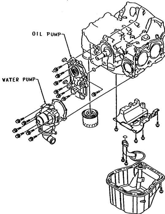
Fig. 21 Layout of water pump and oil pump
