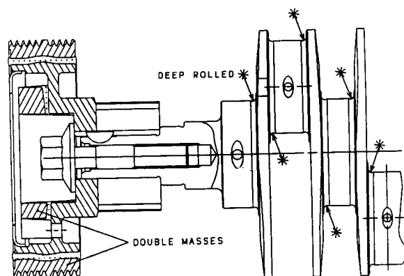
Fig. 5 Fillet roll and double mass damper
