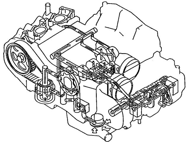
Fig. 22 Lubrication system
