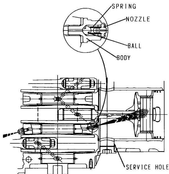
Fig. 10 Service hole and oil jet
