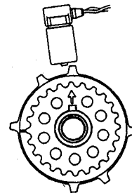
Fig. 26 Crank angle sensor
