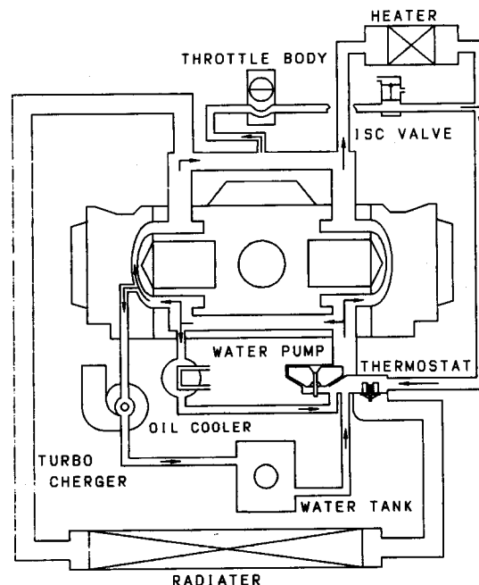
Fig. 20 Cooling system DOHC with turbo
