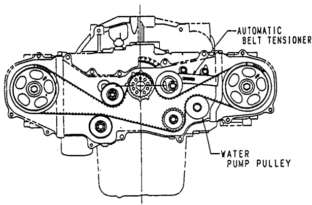
Fig. 18 Camshaft drive system
