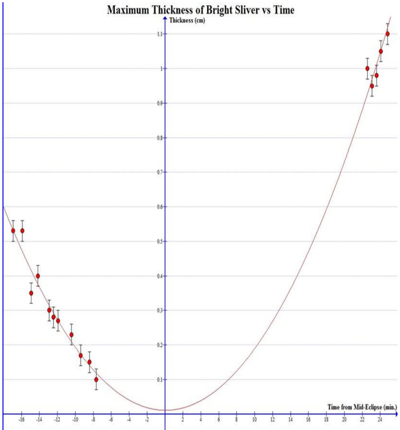
Figure 1 - 2015 April 4 Lunar Eclipse, Maximum Thickness of Bright Sliver as Function of Time (by Helio C. Vital)
