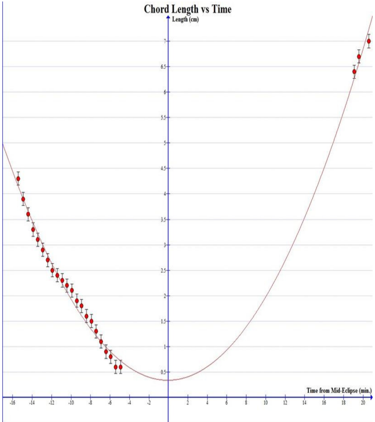
Figure 2 - 2015 April 4 Lunar Eclipse, Chord Length of Bright Sliver as Function of Time (by Helio C. Vital)
