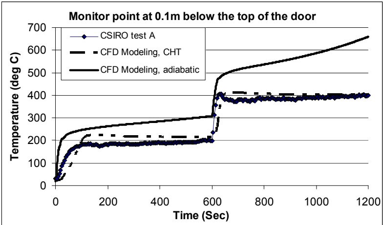
Figure 8: Gas temperature obtained with different boundary condition for case A
