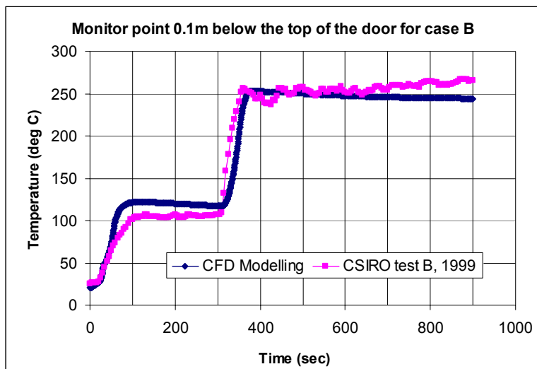
Fig 10: Gas temperature at 0.1m below the top of the door centre for case B
