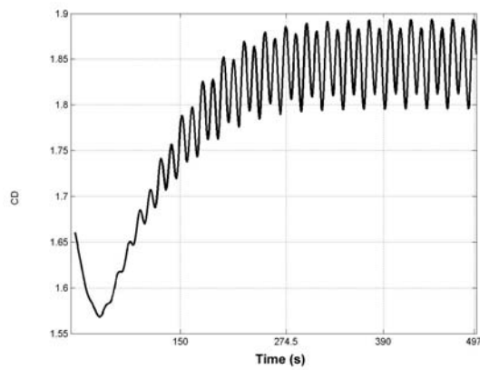
Figure 6a: Drag force coefficient C_D
