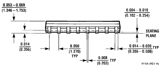
16-Lead Small Outline Molded Package (M) Order Number DM74LS75M NS Package Number M16A
