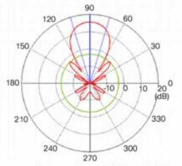
Antenna Azimuth Plane Pattern
