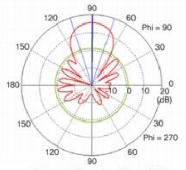
Antenna Elevation Plane Pattern
