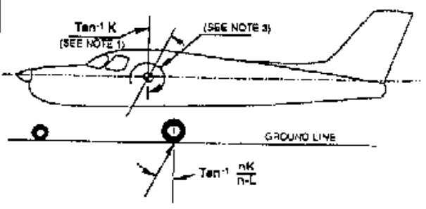
LEVEL LANDING WITH NOSE WHEEL JUST CLEAR OF GROUND
