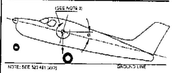
TAIL DOWN LANDING
