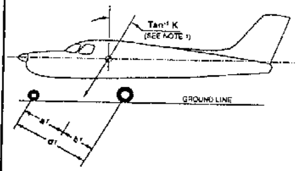
LEVEL LANDING WITH INCLINED REACTIONS
