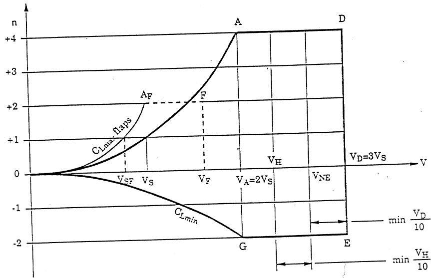
Figure 3 - Flight Envelope
