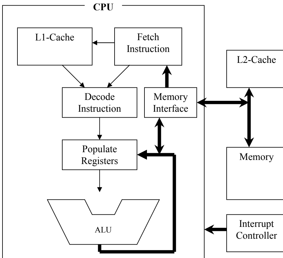
Fig 1.2.1: CPU Architecture
