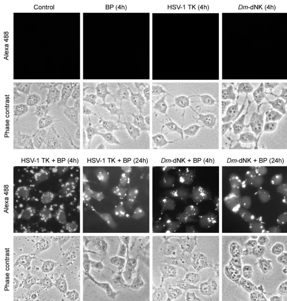
Fig. 1. Liposome-mediated import of nucleoside kinases in a osteosarcoma cell line. The cells were incubated with recombinant fluorescent Alexa Fluor-488-labeled HSV-1 TK or Dm -dNK alone or in complex with BioPorter (BP) lipids for 4 or 24 h. The cells were thoroughly washed after incubation, and fluorescence microscopy was performed on the live unfixed cells.
