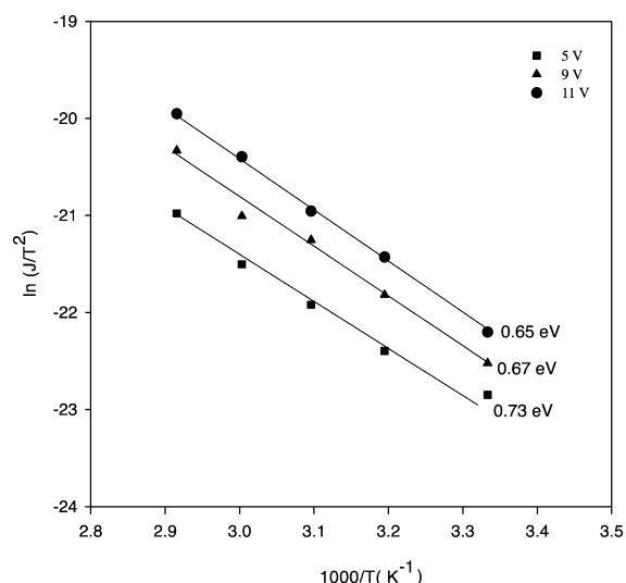
Fig. 5. Plot of \ln(J/T^2) against 1000/T for Al/polyaniline/Al structure of film thickness 1350 Å for different applied bias voltages.
