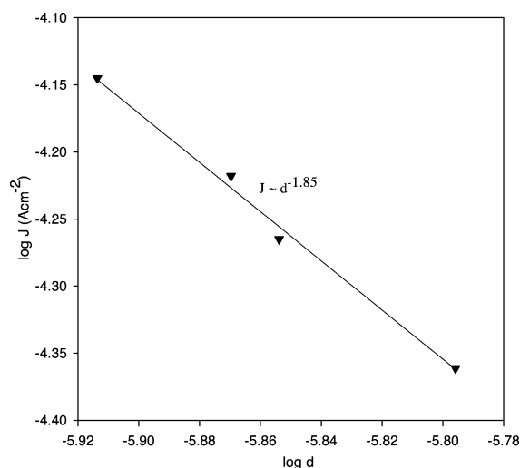
Fig. 2. Thickness dependence on the current density for Al/polyaniline/Al thin film at room temperature.
