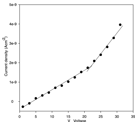
Fig. 1. Current density against applied voltage for Al/polyaniline/Al film of 1350 Å in thickness at room temperature.
