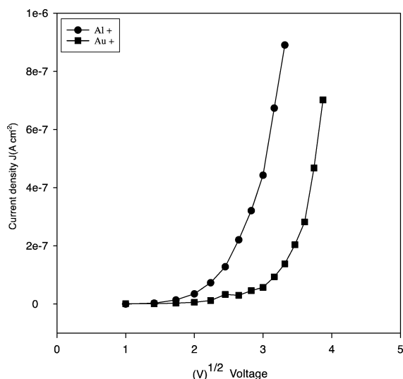
Fig. 4. Schottky plot for Au/polyaniline/Al asymmetric electrode configuration at room temperature.
