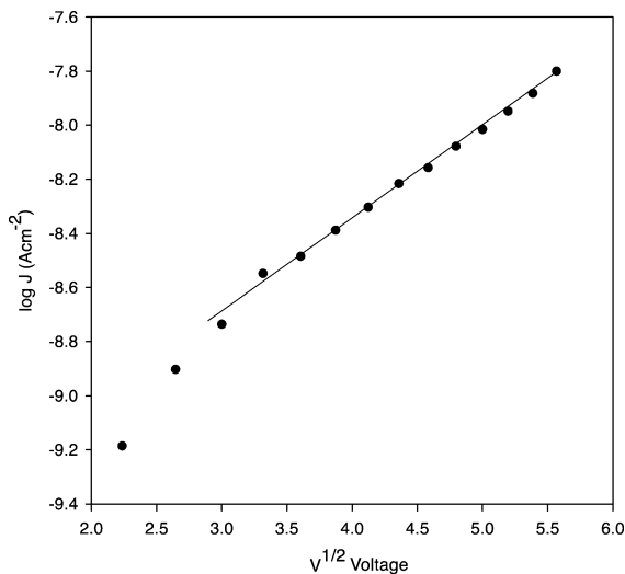
Fig. 3. Schottky plot for Al/polyaniline/Al polymer thin film of thickness 1350 Å.
