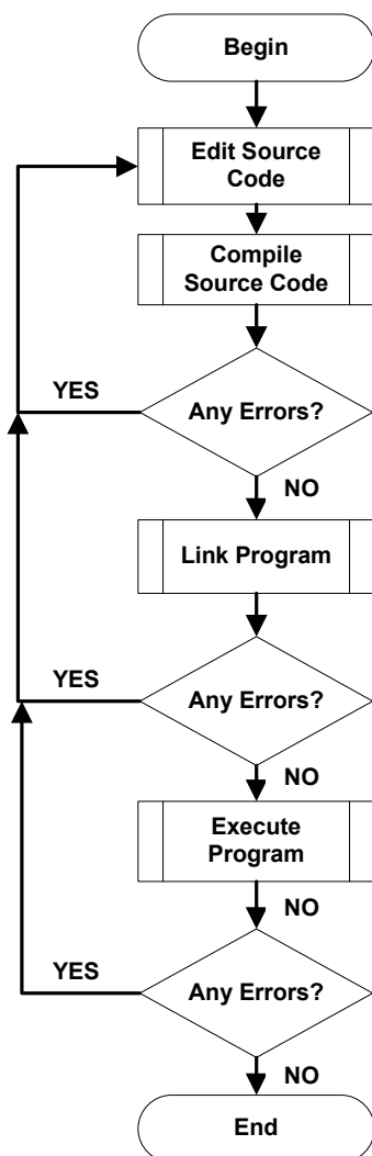
Figure 1 The steps involved in C program development.
