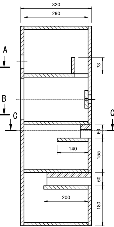
Section EE
