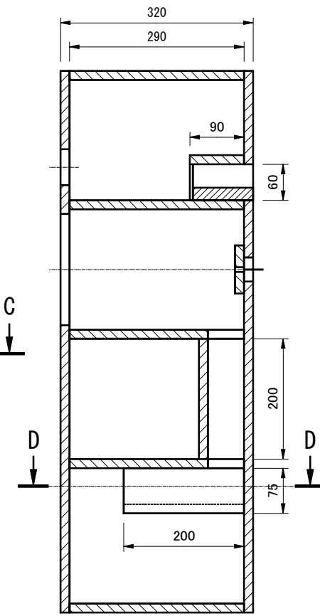
Section FF
