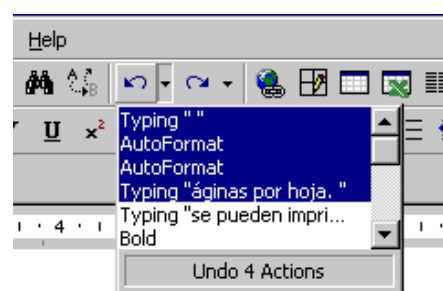
Figura 1. Botón Undo .
