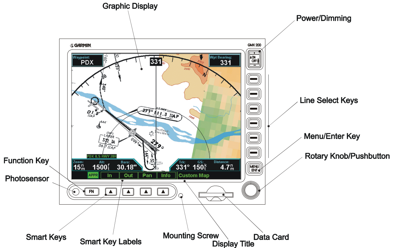
Figure 1-4. GMX 200 Front Panel Description
