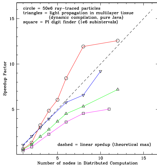
Figure 1. Peak JTS speedups VS sequential GCC -O3
