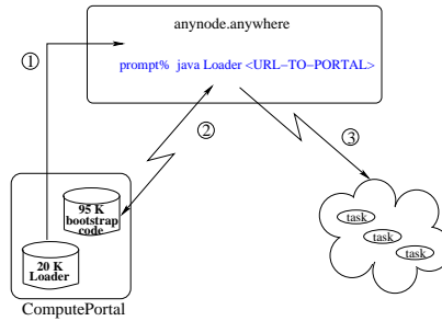
Figure 2. Simplified remote node configuration with JTS.
