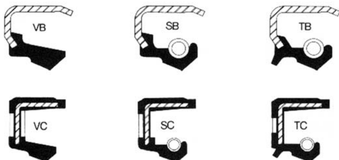
Sample profiles of Oil Seal Styles available below.
