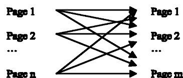
Figure 2 A link structure without a gateway site
