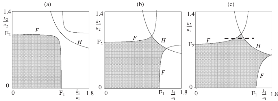
Figure 3. Learning region projected in the two-dimensional plane (K_1/u_1, K_2/u_2) . The shaded area represents the learning region, the bifurcation curves that bound it are equilateral hyperbolas: F denotes the positive branches of the Flip (period doubling) bifurcation curve, H the positive branch of the Neimark-Hopf bifurcation curve. (a) With the set of parameters B=5, \alpha_1=0.5, \alpha_2=0.8 , the condition \alpha_1/2 < \alpha_2 < 2\alpha_1 holds, then the two hyperbolas do not intersect, and the learning region is bounded only by the Flip bifurcation curve; (b) With the set of parameters B=5, \alpha_1=0.5, \alpha_2=1.3 , the two hyperbolas intersect in the positive orthant, so the learning region is bounded by an arc of the Neimark-Hopf bifurcation curve and by two arcs of the flip bifurcation curve; (c) With the set of parameters B=5, \alpha_1=0.3, \alpha_2=1.4 , the arc of the curve H included in the boundary of the stability region becomes more extended.
