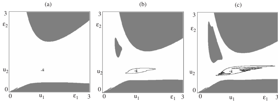
Figure 5. The condition \alpha_1/2 < \alpha_2 < 2\alpha_1 is not satisfied and, consequently, the stability region is also bounded by a portion of the curve H where a Neimark–Hopf bifurcation occurs. (a) Using B=5 , \alpha_1=0.5 , \alpha_2=1.3 (like in figure 3b) and u_1=1.2 , u_2=0.8 , K_1=1.2 , K_2=0.64 , the parameters are inside the stability region and the steady state is a stable focus; (b) B=5 , \alpha_1=0.5 , \alpha_2=1.3 , u_1=1.2 , u_2=0.8 , K_1=1.56 , K_2=0.72 , so that (K_1/u_1, K_2/u_2) is outside of the learning region, close to the boundary H . The steady state is an unstable focus, and an attracting closed invariant curve exists around it; (c) With B=5 , \alpha_1=0.5 , \alpha_2=1.3 , u_1=1.2 , u_2=0.8 , K_1=1.63 , K_2=0.75 , the attractor is a chaotic ring around the unstable focus \bar{\varepsilon} .
