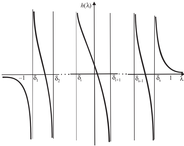
Figure 1. Graphical representation of the function h(\lambda) in the proof of Theorem 2.
