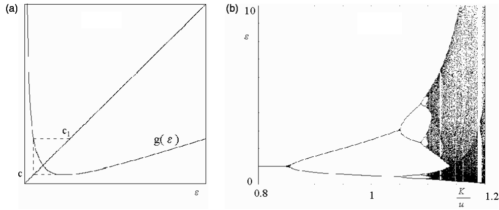
Figure 2. (a) Graphical representation of the map g with the set of parameters B=5, K=1, \alpha=1, n=2, u=1 . As far as the minimum value c=f(x_{\min}) > 0 , the asymptotic dynamics are trapped inside the interval [c, c_1] , where c_1=f(c) is the rank-1 image of the minimum point. (b) Bifurcation diagram for the one-dimensional map g with the same parameters B=5, \alpha=1, n=2 and K/u as a bifurcation parameter in the range [0.8, 1.2] .
