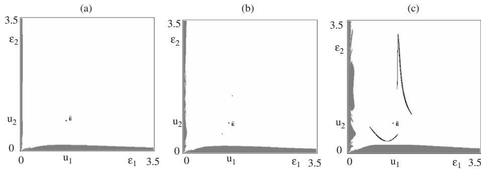
Figure 4. The white region represents the set of points that generate feasible trajectories (i.e. trajectories entirely included inside the positive orthant) and converging to the steady state, or another attractor around it, whereas the grey region represents the set of points that generate unfeasible trajectories. (a) With B=5 , \alpha_1=0.5 , \alpha_2=0.8 (like in figure 3b) and u_1=1.2 , u_2=0.8 , K_1=0.6 , K_2=0.7 , the parameters are inside the stability region and the steady state is a stable node; (b) With B=5 , \alpha_1=0.5 , \alpha_2=0.8 , u_1=1.2 , u_2=0.8 , K_1=0.6 , K_2=0.9 , the parameters are outside the region of stability (close to the boundary F , see figure 3a), the steady state is a saddle point, and the only attractor is a stable cycle of period 2, represented by the two small dots; (c) With B=5 , \alpha_1=0.5 , \alpha_2=0.8 , u_1=1.2 , u_2=0.8 , K_1=0.6 , K_2=1.05 , a chaotic attractor exist.
