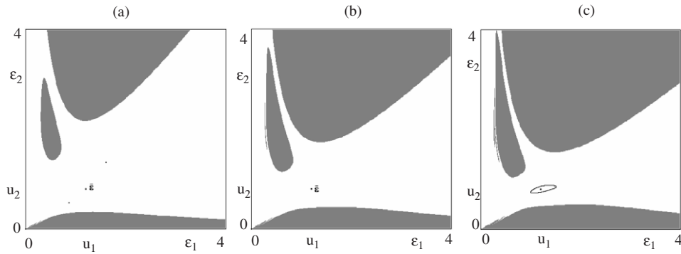
Figure 6. Qualitative changes of long-run behaviour of the learning process when the heterogeneity condition (36) holds. Effects of increasing values of K_1/u_1 and/or K_2/u_2 when we follow the bifurcation path, in the space of parameters, represented by the dashed line in figure 3c. (a) With B=5 , \alpha_1=0.3 , \alpha_2=1.4 , u_1=1.2 , u_2=0.8 , K_1=0.84 , K_2=0.7 , the learning process approaches, in the long run, a stable cycle of period 2; (b) With the same set of parameters, but increasing the value of K_1 ( K_1=1.2 ), the learning process converges to the true demand (i.e. the parameters are inside the learning region); (c) This figure is obtained after a further increase of the speed of adjustment K_1 ( K_1=1.44 ). The steady state is again unstable and the long-run dynamics of the learning process are characterized by quasi-periodic oscillations along a stable close invariant orbit around the unstable steady-state.
