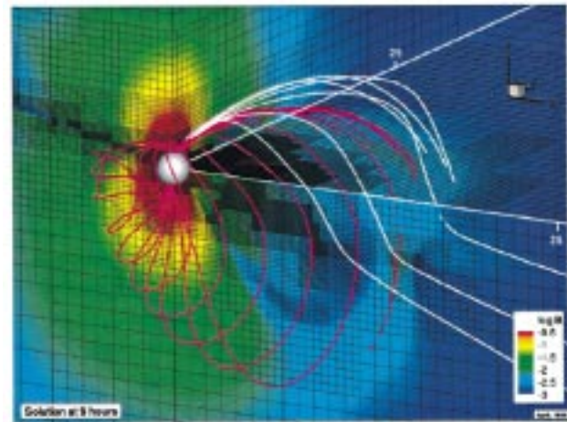
Fig. 7. Simulation of a coronal mass ejection (CME) illustrating the 3-D adapted grid structure to resolve multiple-scale phenomena. Magenta lines represent compressed closed field lines ahead of the CME, while white lines show the distorted structure of open magnetic field lines. The color code represents \log(B) .
