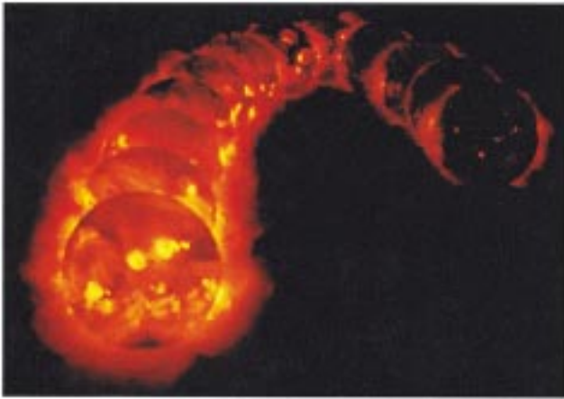
Fig. 1. The 12 X-ray images of the Sun obtained by the Yohkoh satellite between 1991 (left) and 1995 (right) at 90-day increments provide a dramatic view of how the solar corona changes from solar maximum to solar minimum. As we approach solar maximum anticipated in 2001 or 2002, the reverse progression will occur. (Figure courtesy of Lockheed Martin.)
