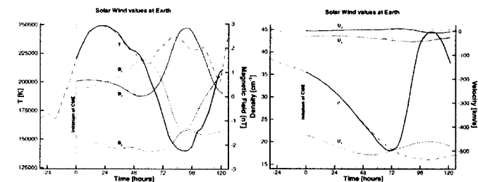
Fig. 8. Simulated solar wind parameters at the Earth—Dashed lines: without CME, solid lines: with CME.
