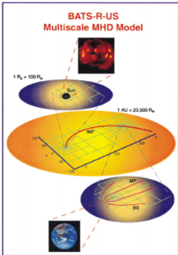
Fig. 6. The Michigan MHD Model. Note that the model spans multiple scales, from a few hundred kilometers in the ionosphere to the radius of the Earth ( R_E ), to the radius of the Sun ( R_S ), to the Sun–Earth distance (AU).
