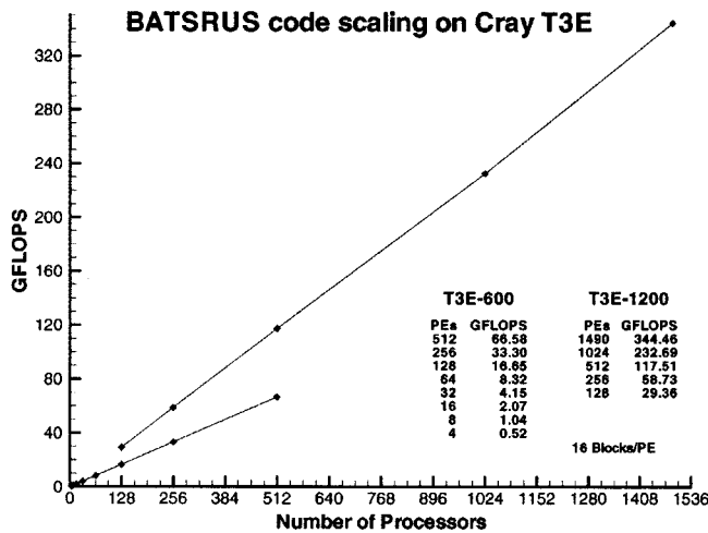
Fig. 4. Parallel scaling of the BATSRUS code.
