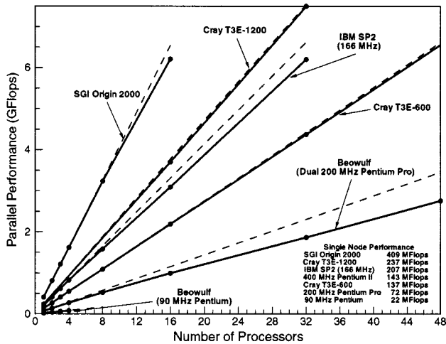
Fig. 5. Parallel performance of BATSRUS code for a variety of parallel architectures. The dashed line indicates ideal scale-up performance based on single node performance and solid lines indicate actual performance achieved on each of the machines.
