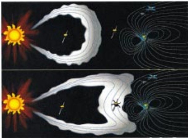
Fig. 2. The interaction of the magnetosphere with an expanding magnetic cloud. (Illustration courtesy of the NASA International Solar Terrestrial Program.)
