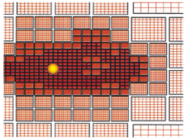
Fig. 3. Adapted grid in the simulation of a coronal mass ejection. The figure shows a 2-D cross section of the 3-D grid structure (cutting through the CME).
