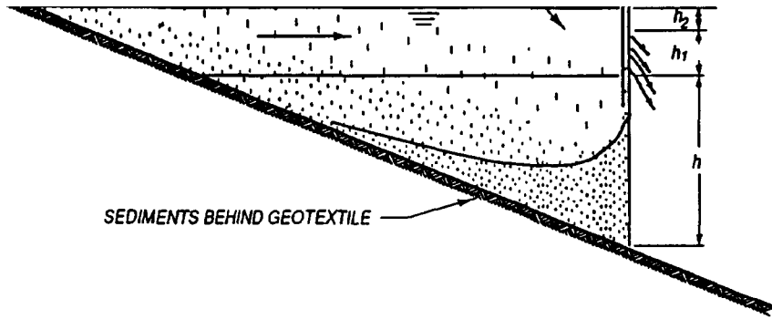
Figure 6-7. Sedimentation behind Silt Fence.
