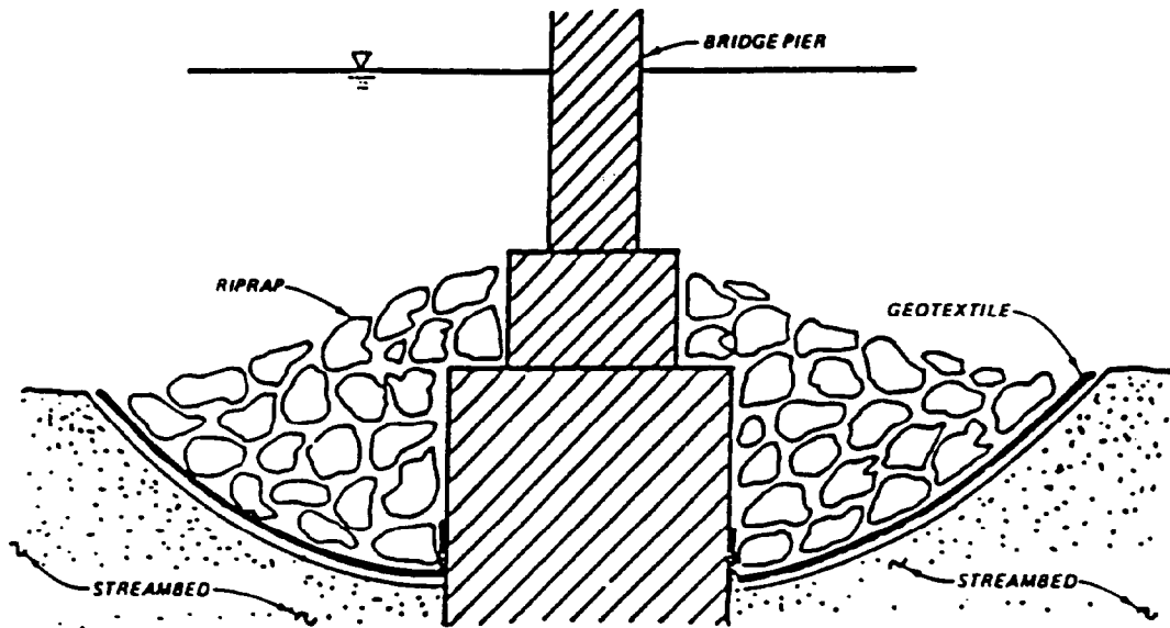
SCOUR PROTECTION FOR BRIDGE PIER
