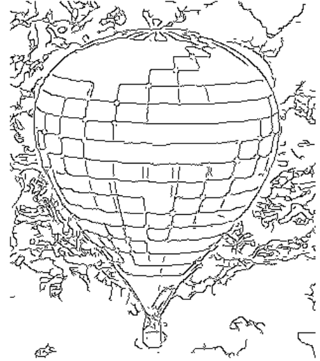
Fig. 10. Result using Ruzon et al. 's method on balloon image shown in Fig. 4(c) with R = 1.5 , low = 0.1 , high = 0.46
