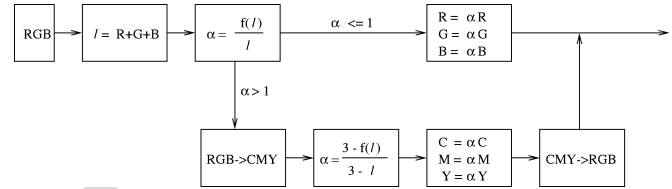
Fig. 4. Block diagram of the proposed enhancement scheme.
