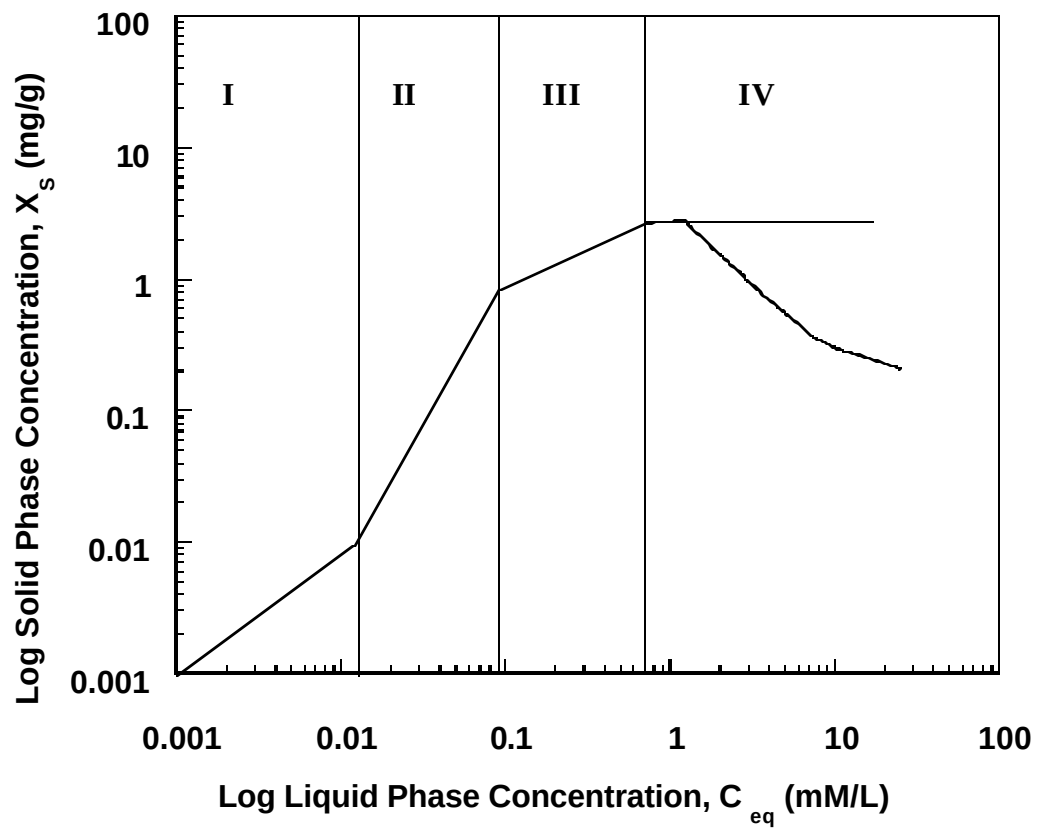
Figure-2.3: Schematic presentation of typical four-regime adsorption isotherm.
