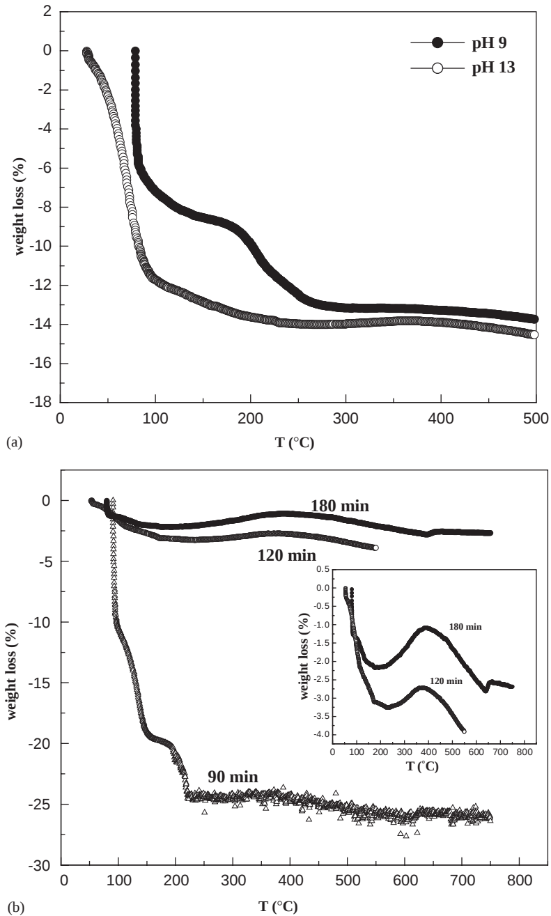
Fig. 1. (a) TGA plot of air-dried Mn-ferrite prepared at different pH (9 and 13) with a fixed refluxing time of 30 min. (b) TGA plot of Mn-ferrite prepared at different refluxing times at fixed pH 11. The inset is a magnified TGA plot of the samples with refluxing times of 120 and 180 min.
