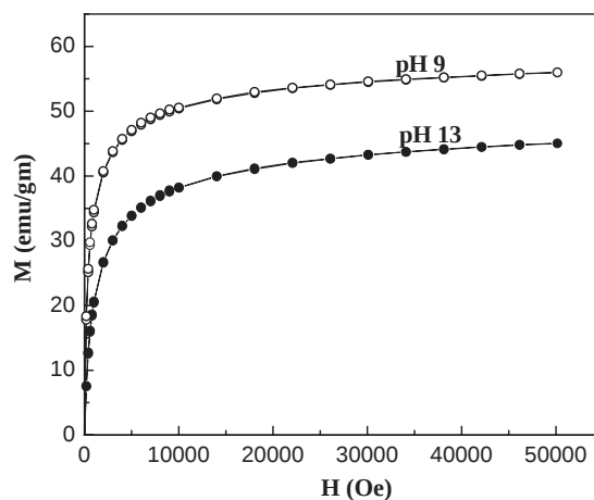
Fig. 4. Magnetization vs. field plots of sample prepared at different pH with a fixed refluxing time of 30 min.
