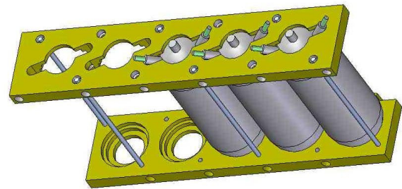
Gambar 2. Mounting baterai
