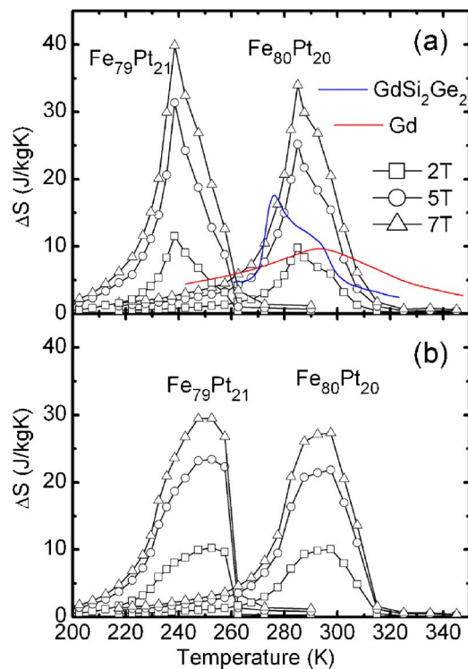
FIG. 5. (Color online) Magnetic entropy change |\Delta S| of Fe 79 Pt 21 and Fe 80 Pt 20 alloys for the magnetic field changes of 0–2, 0–5, and 0–7 T with (a) increasing field and (b) decreasing field, respectively. For comparison, the |\Delta S| of Gd and Gd 5 Ge 2 Si 2 under 0–5 T are also presented which are quoted from Refs. 6 and 7.
