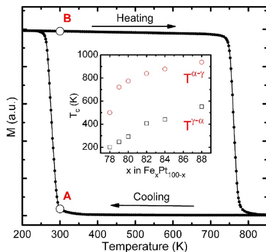
FIG. 1. (Color online) Thermomagnetic curves of the \text{Fe}_{80}\text{Pt}_{20} alloy under 100 Oe magnetic field. The inset gives the dependence of T^{\alpha \rightarrow \gamma} and T^{\gamma \rightarrow \alpha} on x in \text{Fe}_x\text{Pt}_{100-x} alloys.
