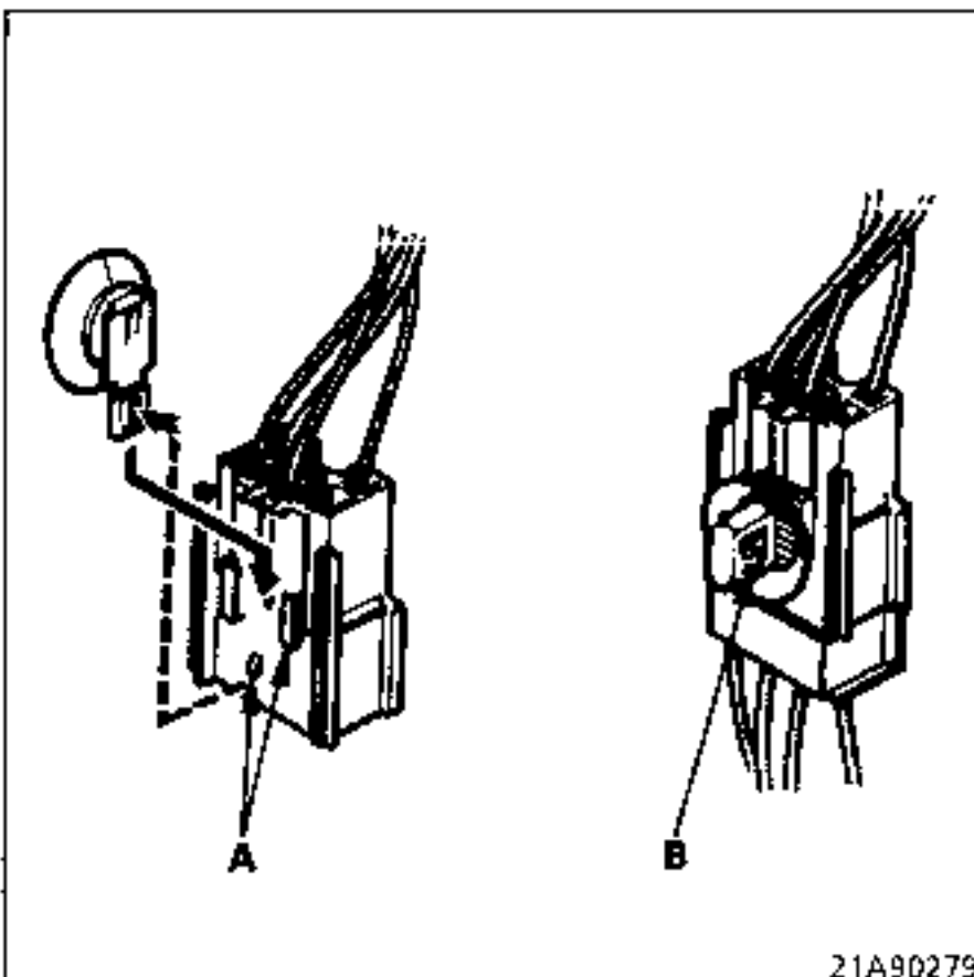
A Female socket mounting on door
