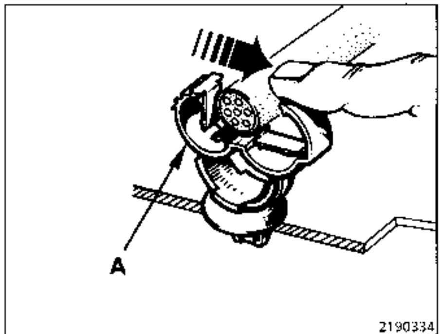
Harness mounting clip.
