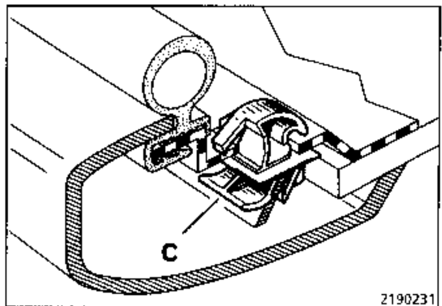
(C) Snap mounting
