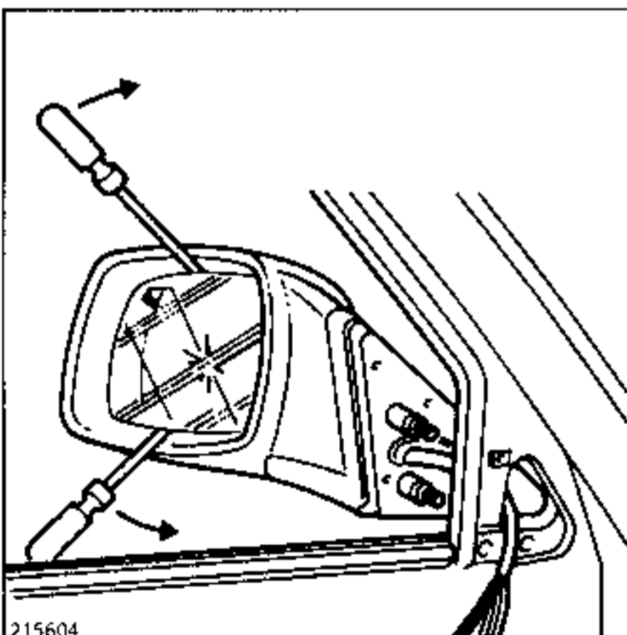
Method for removing a damaged mirror glass.
