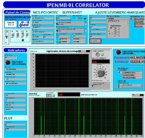
FIG. 3: The IPEN/MB-01 Correlator front panel.
