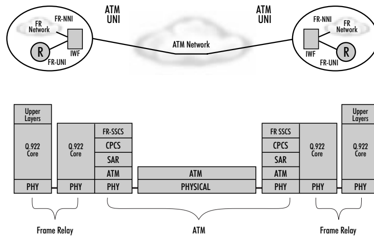
Figure 23: Frame/ATM Network Interworking (Encapsulation)
