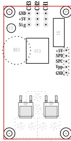
Bottom/trace side
