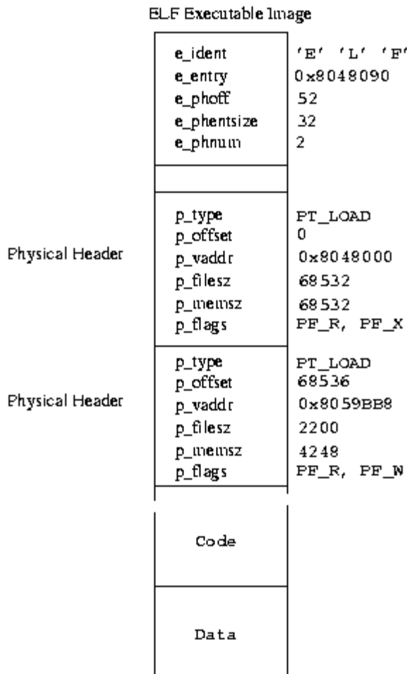
Figure 4.4: ELF Executable File Format
