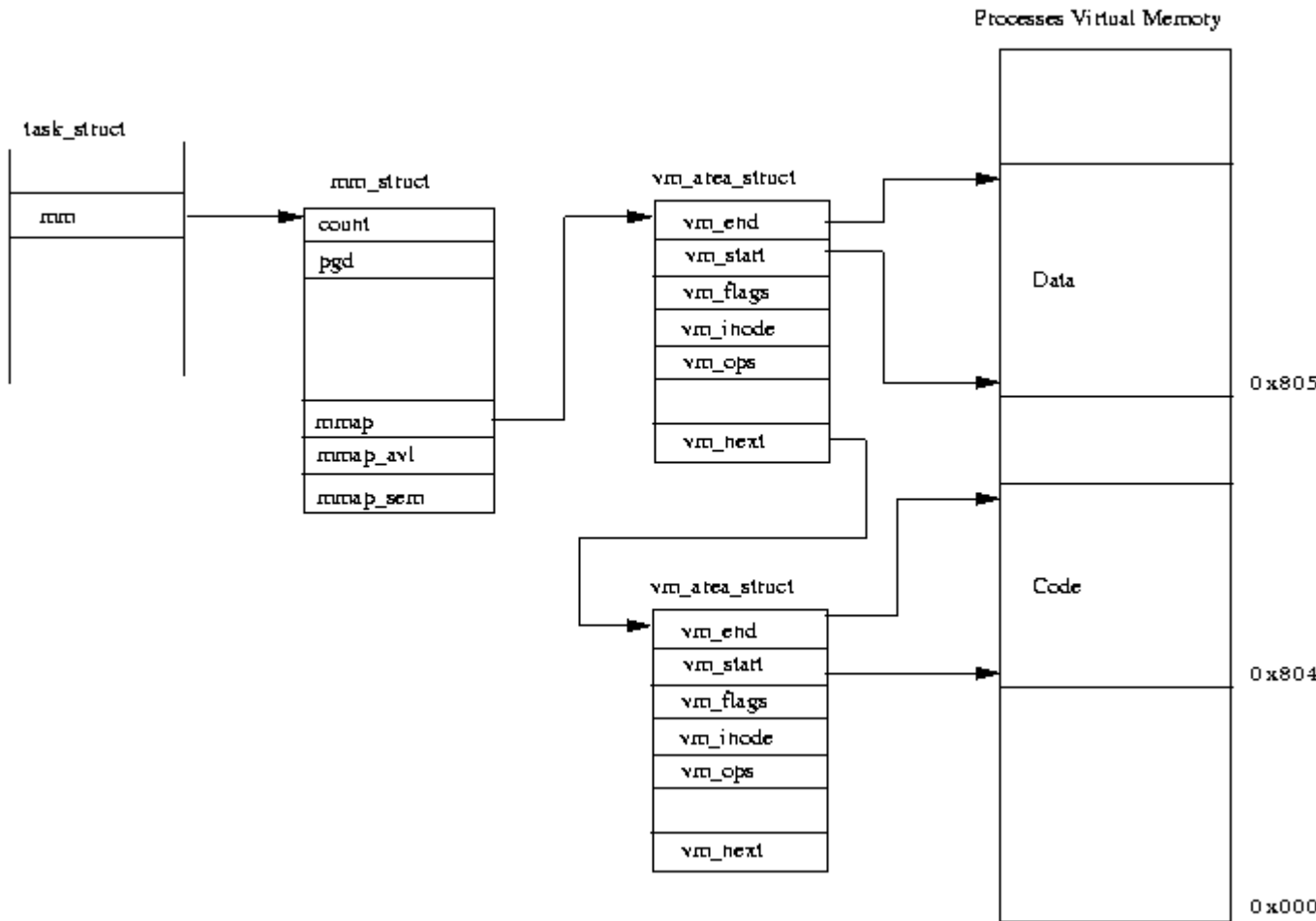
Figure 4.2: A Process's Virtual Memory
