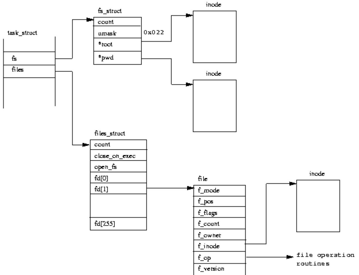
Figure 4.1: A Process's Files
