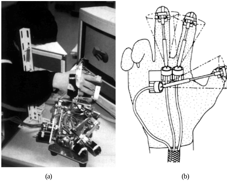
Figure 2.5.2.1. Force feedback hand masters: (a) Master Manipulator (from [Iwat90]), (b) force feedback structure for the data glove (from [Burd92]).
