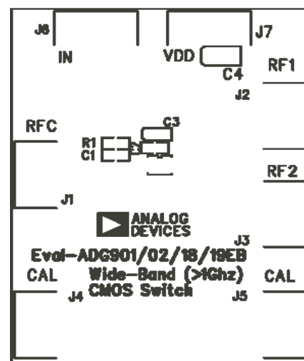
Figure 6. ADG9xx Evaluation Board Top View
