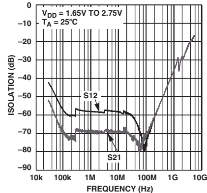
TPC 5. Isolation vs. Frequency over Supplies (RF1/RF2, ADG918)
