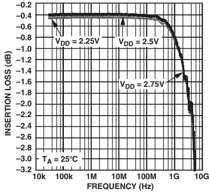
TPC 1. Insertion Loss vs. Frequency over Supplies (RF1/RF2, S12, and S21)
