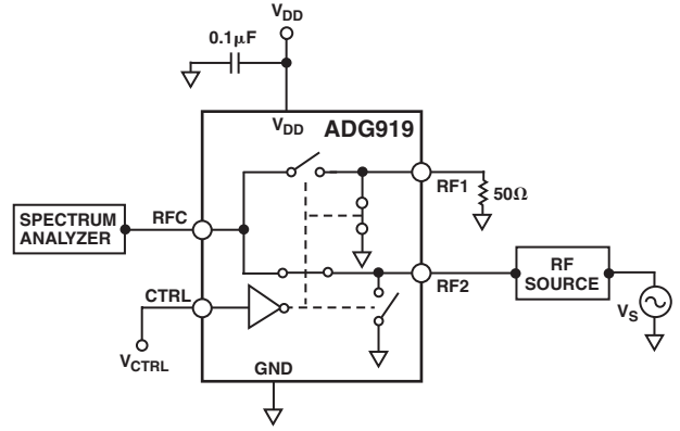
Test Circuit 8. P_{-1dB}
