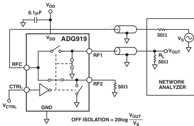
Test Circuit 3. Off Isolation
