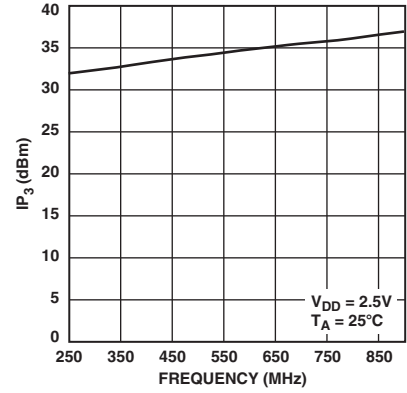
TPC 12. IP_3 vs. Frequency
