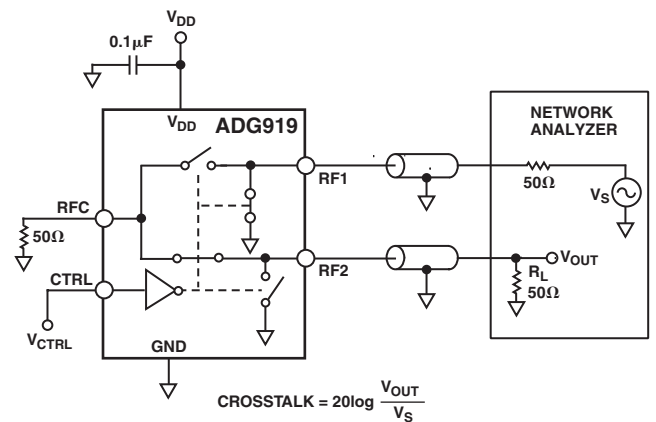
Test Circuit 5. Crosstalk
