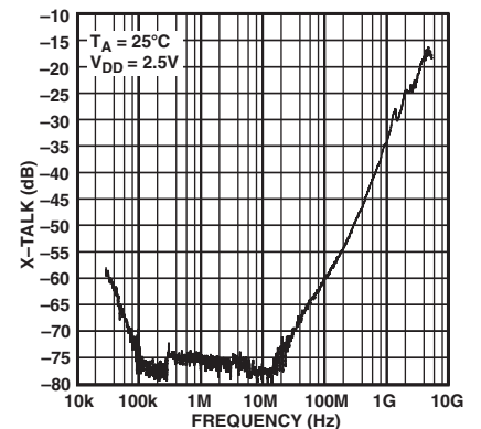
TPC 9. Crosstalk vs. Frequency (RF1/RF2, S12, S21)
