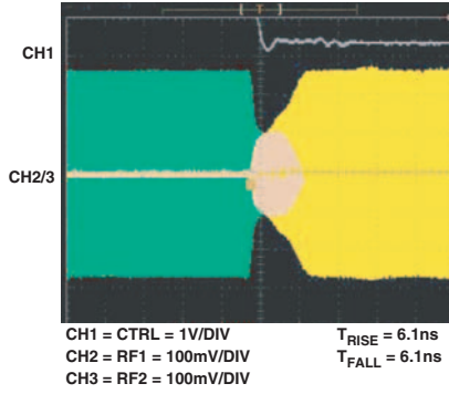
TPC 10. Switch Timing
