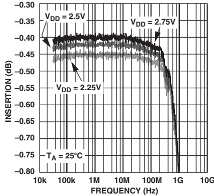
TPC 2. Insertion Loss vs. Frequency over Supplies (RF1/RF2, S12, and S21) (Zoomed TPC 1 Plot)
