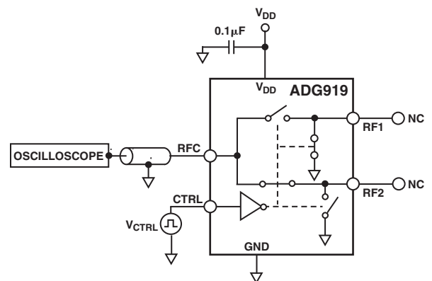
Test Circuit 6. Video Feedthrough
