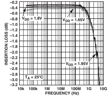
TPC 3. Insertion Loss vs. Frequency over Supplies (RF1/RF2, S12, and S21)
