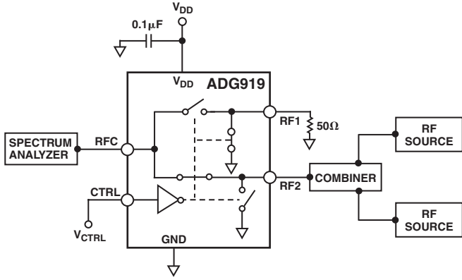
Test Circuit 7. IP_3
