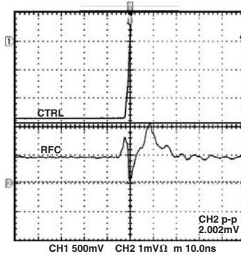
TPC 11. Video Feedthrough
