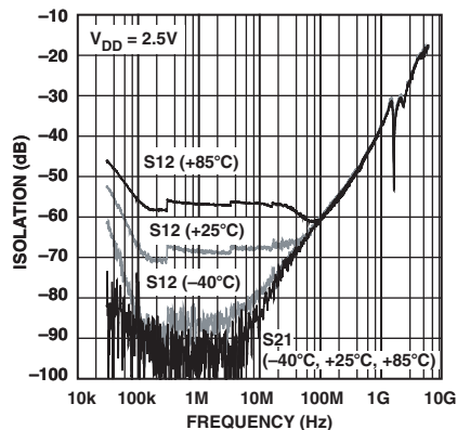
TPC 7. Isolation vs. Frequency over Temperature (RF1/RF2, ADG919)
