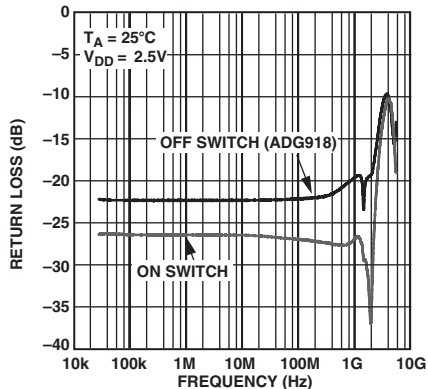
TPC 8. Return Loss vs. Frequency (RF1/RF2, S11)
