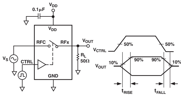
Test Circuit 2. Switch Timing: t_{RISE} , t_{FALL}
