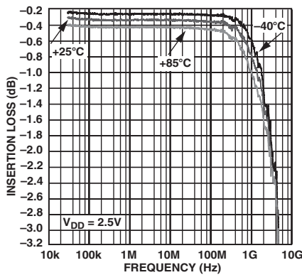
TPC 4. Insertion Loss vs. Frequency over Temperature (RF1/RF2, S12, and S21)
