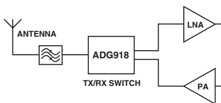
Figure 3. Wireless Metering
