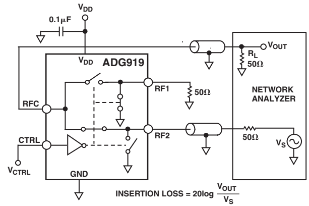
Test Circuit 4. Insertion Loss
