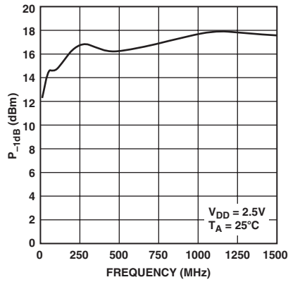
TPC 13. P_{-1dB} vs. Frequency
