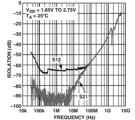
TPC 6. Isolation vs. Frequency over Supplies (RF1/RF2, ADG919)
