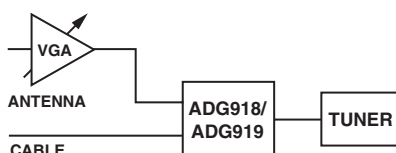
Figure 4. Tuner Modules
