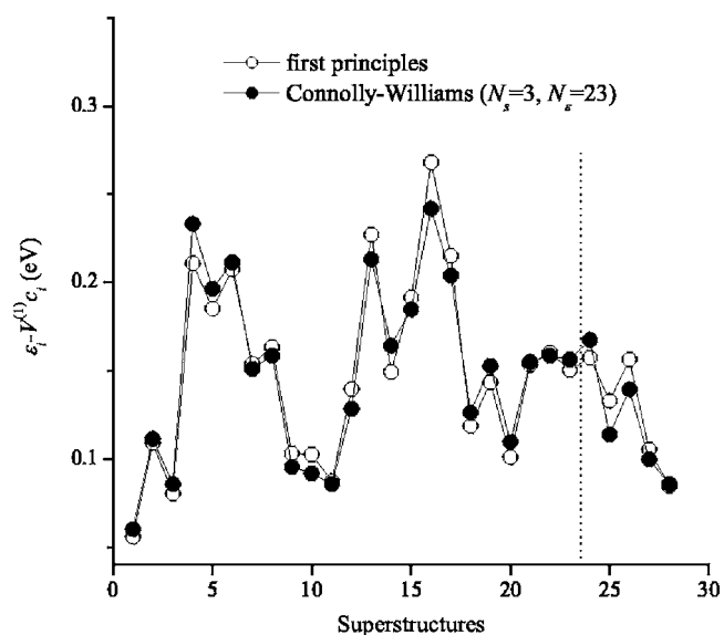
FIG. 4. The values of \varepsilon_i - V^{(1)}c_i [see Eqs. (9) and (10)] for 28 equiatomic ( c_i=0.5 ) structures calculated both directly from first principles and by the use of the mixing potentials obtained by the Connolly-Williams method (at N_s=3, N_e=23 ). The differences between those two energies characterize the accuracy of Connolly-Williams fitting in the case of each structure. The first 23 structures (see the Appendix) are linearly independent and they (and only they) were used in the Connolly-Williams method. The last 5 structures (right side of the vertical dashed line) correspond to all distinguishable (but not identical to the previous 23 ones) equiatomic structures based on two-cubic unit cells in the fcc crystal lattice (see the Appendix). Those 5 structures were not used in the Connolly-Williams fitting, but they were considered in order to assess the predictive power of the obtained Connolly-Williams potentials.
