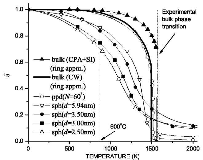
FIG. 11. The temperature dependence of the FePt equilibrium L1_0 order parameter \bar{\eta} obtained within the analytical ring approximation (Ref. 18) for bulk (“bulk”) using KKR-CPA plus strain-induced interactions at L=-0.0294 (CPA+SI) and Connolly-Williams mixing potential at N_s=3, N_e=23 (CW) as well as by Monte Carlo simulation for the parallelepiped (“ppd”) sample containing N=60^3 atoms and for spherical (“sph”) nanoparticles with 2.5, 3.0, 3.5, and 6.0 nm diameters d at equiatomic (or near equiatomic; see Table IV) concentration c=0.5 using Connolly-Williams mixing potential.
