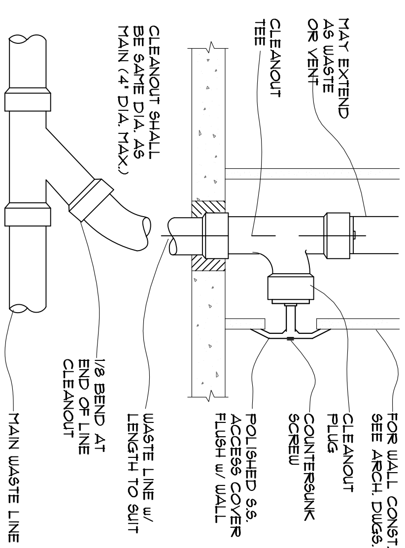
Ø4 WALL CLEANOUT DETAIL
