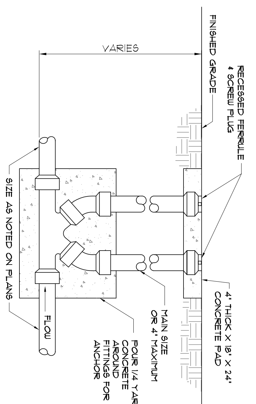
Ø3 TWO-WAY GRADE CLEANOUT DETAIL
