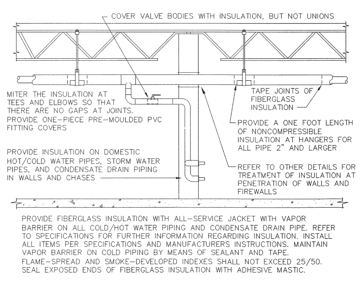
1 PIPE INSULATION SCALE: NO SCALE
