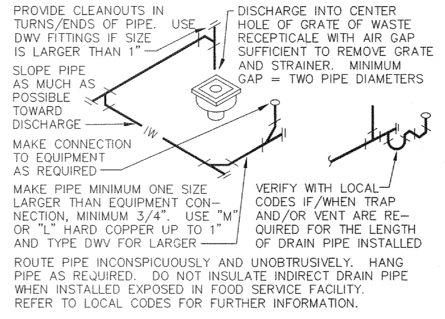
4 INDIRECT DRAIN SCALE: NO SCALE
