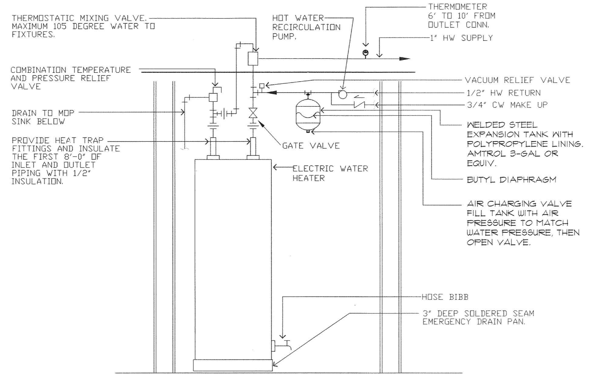
3 WATER HEATER DETAIL SCALE: NO SCALE
