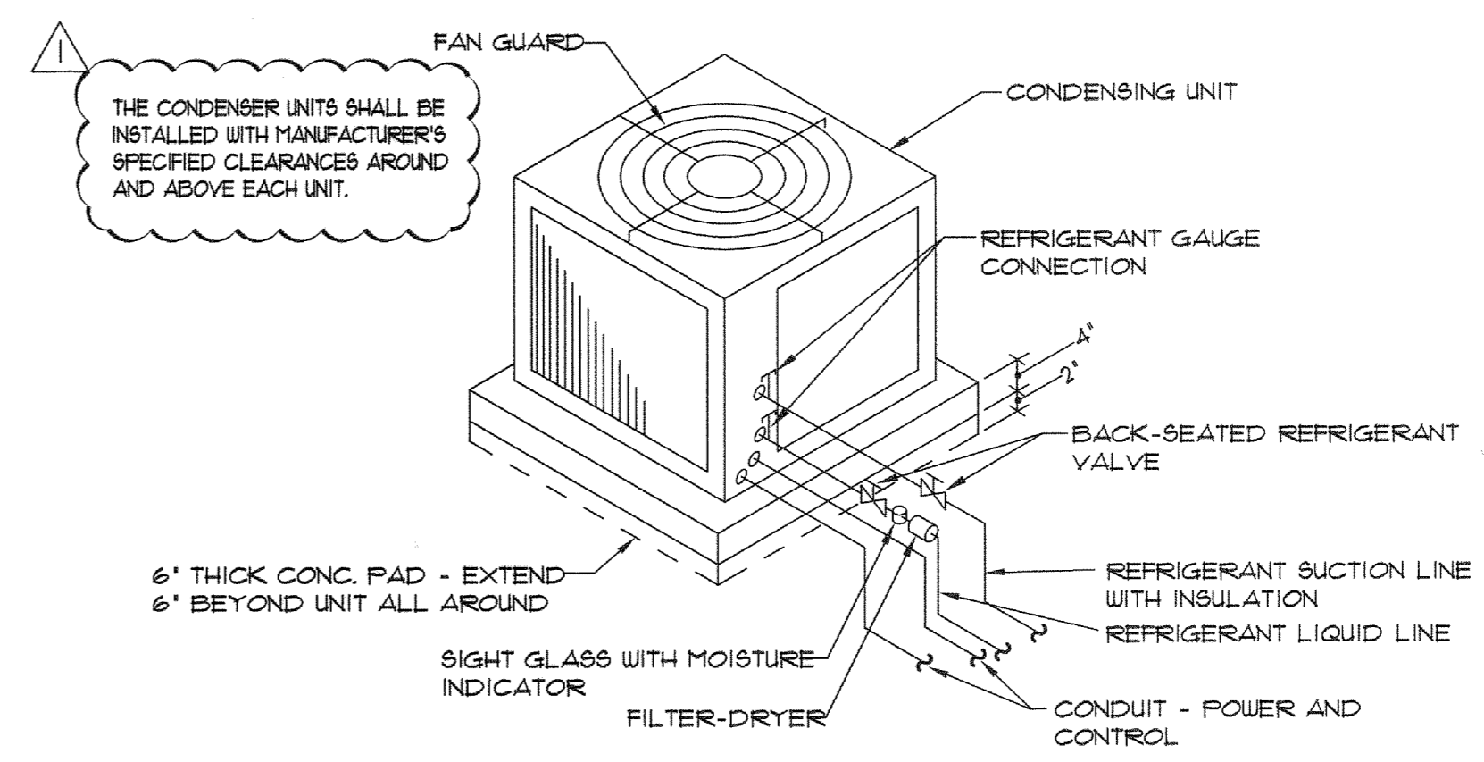
3 CONDENSING UNIT DETAIL SCALE: NO SCALE
