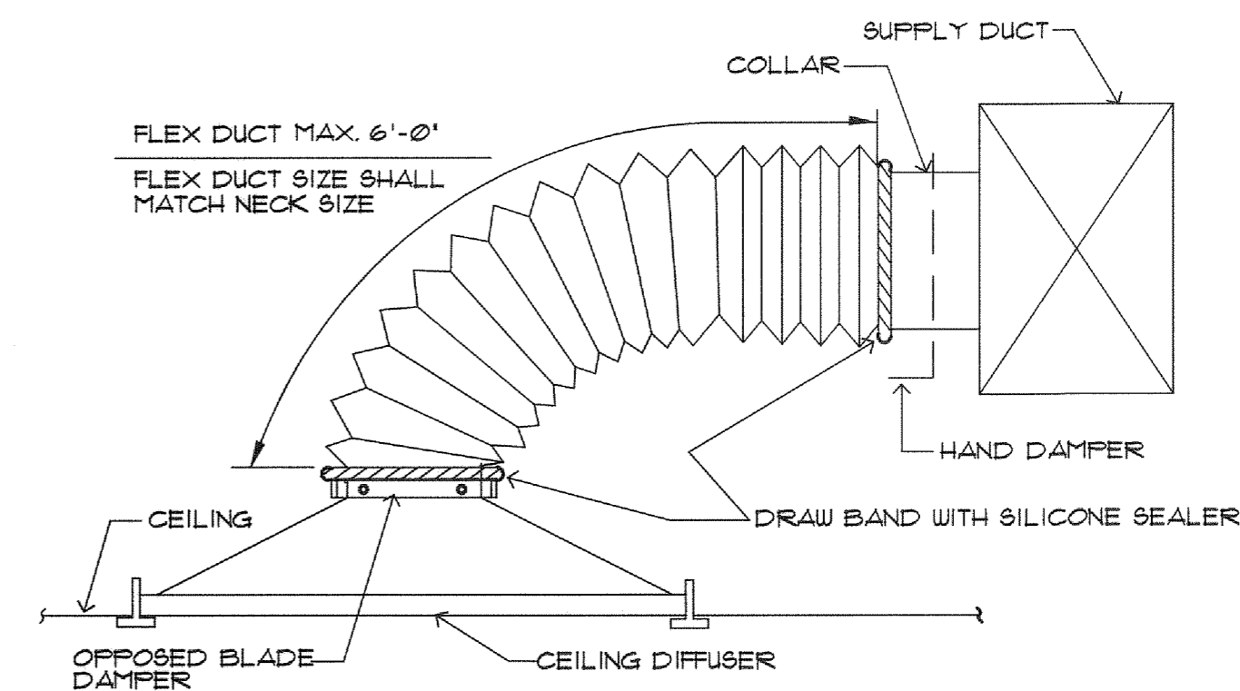
1 TYPICAL DIFFUSER/RETURN GRILLE SCALE: NO SCALE
