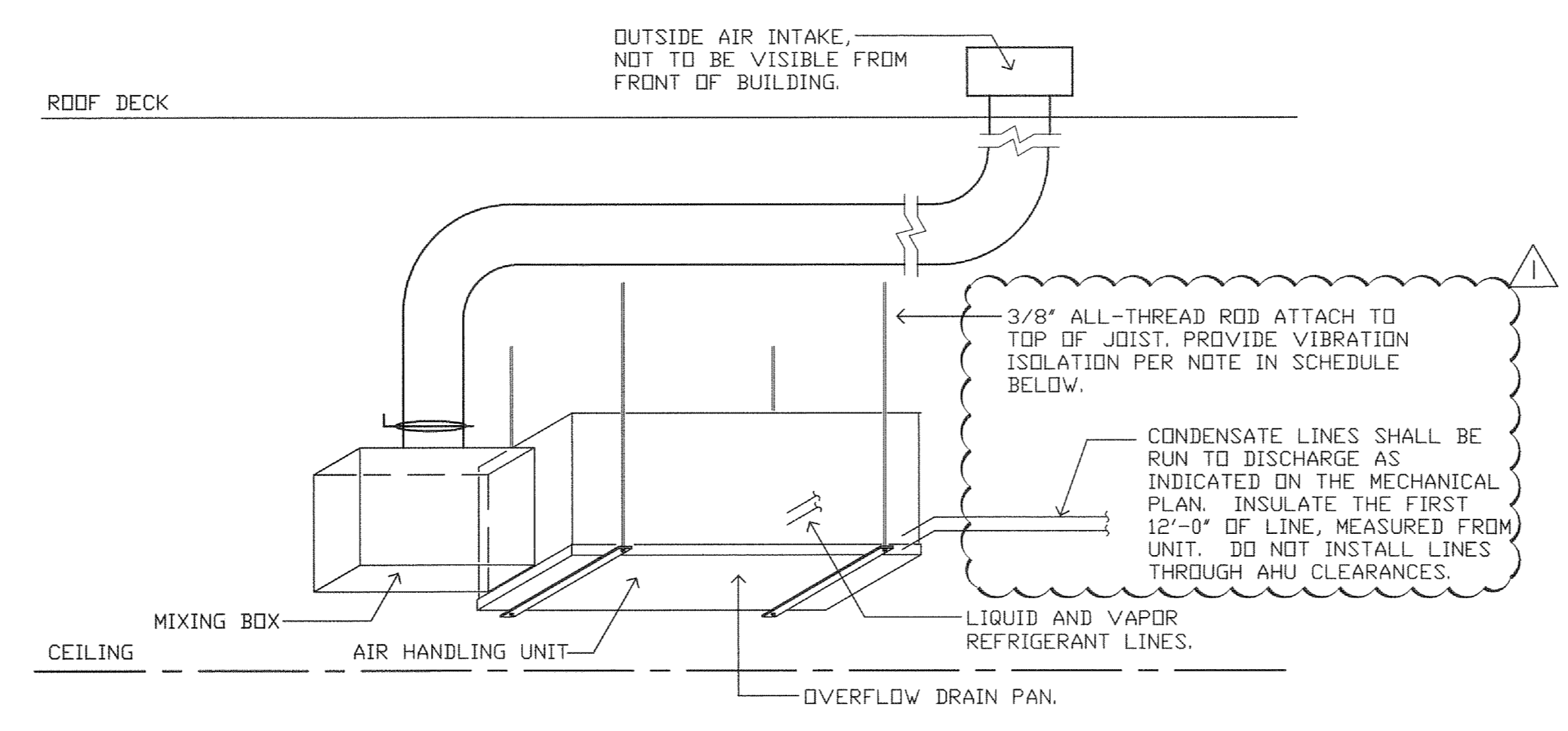
2 AIR HANDLING UNIT DETAIL SCALE: NO SCALE
