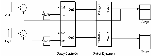
Figure 1 - Block Diagram of an uncompensated Fuzzy Logic Controller for the position control of a two-link robotic manipulator.
