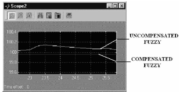
Figure 9 - Zoomed graph to show the relatively large deviation of the control variable from the SP in the case of uncompensated fuzzy logic controller as compared with a compensated fuzzy logic model.
