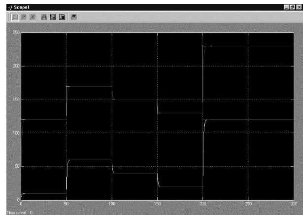
Figure 5a - Multi-Step Response for joint 1(top) and joint 2 of the manipulator controlled using Compensated Fuzzy-Logic Controller.
