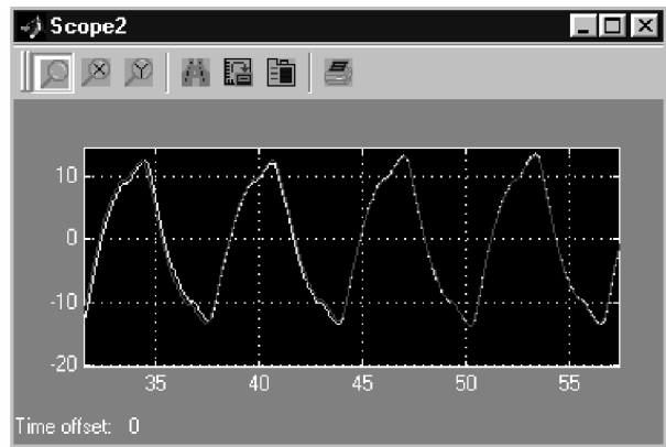
Figure 6 - Sinusoidal Response for the Compensated fuzzy logic Controller. (Sine amplitude =10)
