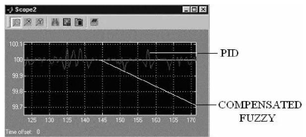
Figure 7 - Response for a load disturbance (step magnitude=10% SP) introduced after the initial step response settling time.
