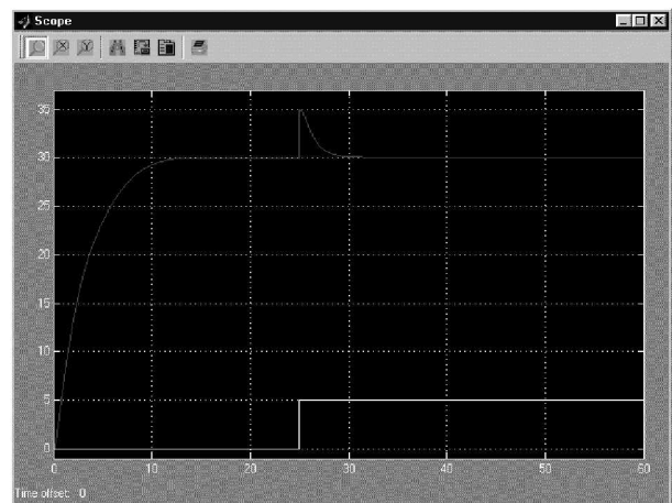
Figure 7 - Response for a load disturbance (step magnitude=10% SP) introduced after the initial step response settling time.
