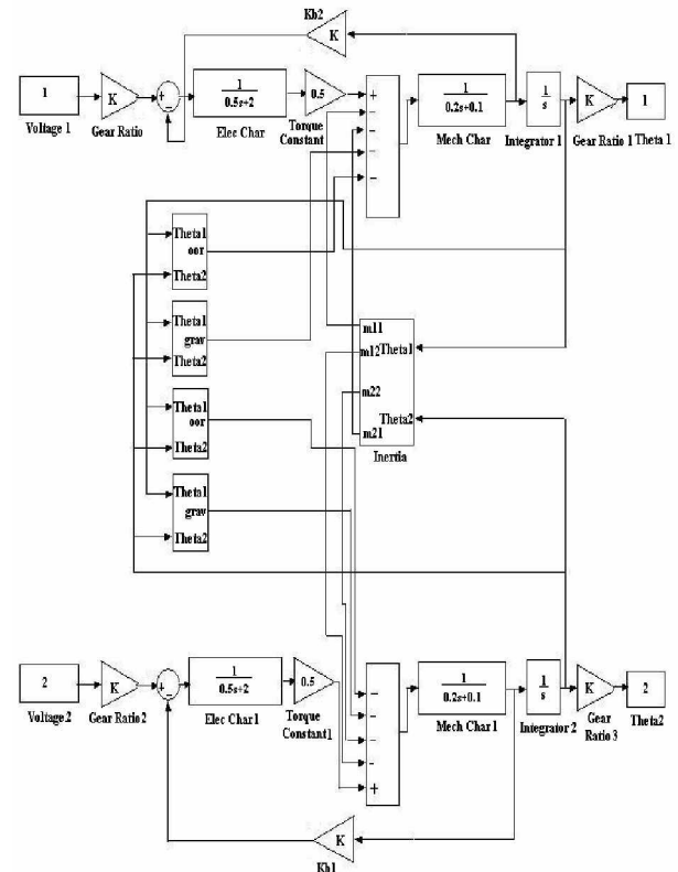
Figure 4 - Dynamic Model of the Two-link robotic manipulator.
