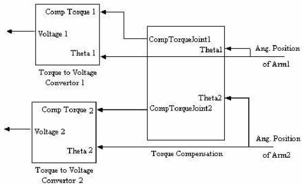
Figure 3 - C-Logic block
