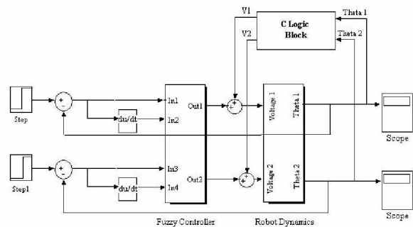
Figure 2 - Block Diagram of the Compensated Fuzzy Logic Controller for the position control of a two-link robotic manipulator as implemented with SIMULINK
