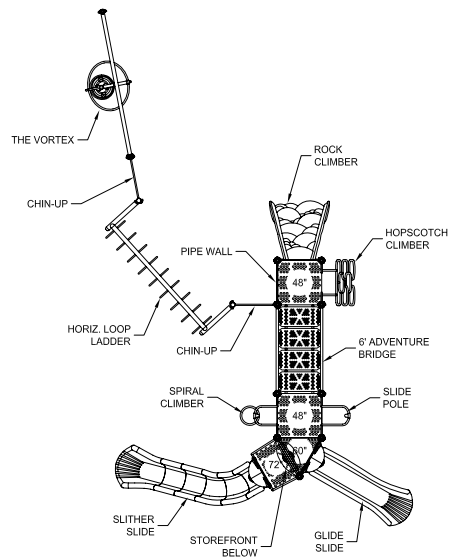
STRUCTURE DETAIL
