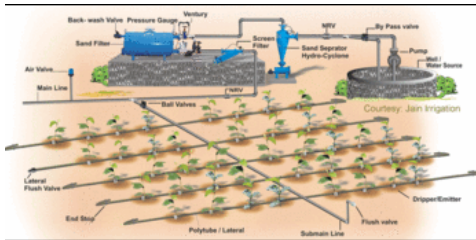
Figure 1: Drip irrigation
