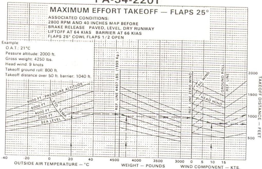
MAXIMUM EFFORT TAKEOFF - 25° FLAPS Figure 5-11
