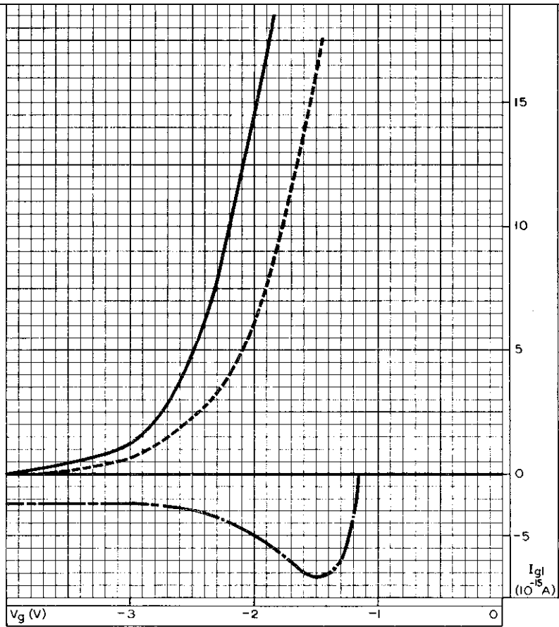
ANODE, SCREEN-GRID AND CONTROL-GRID CURRENTS PLOTTED AGAINST CONTROL-GRID VOLTAGE. V_a = 10V , V_{g2} = 6.5V
