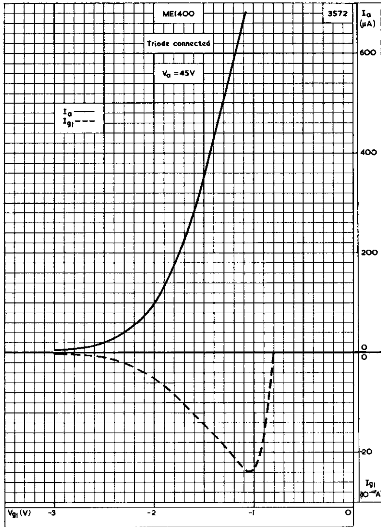
ANODE AND CONTROL-GRID CURRENT PLOTTED AGAINST CONTROL-GRID VOLTAGE. TRIODE CONNECTED. V_a = 45V
