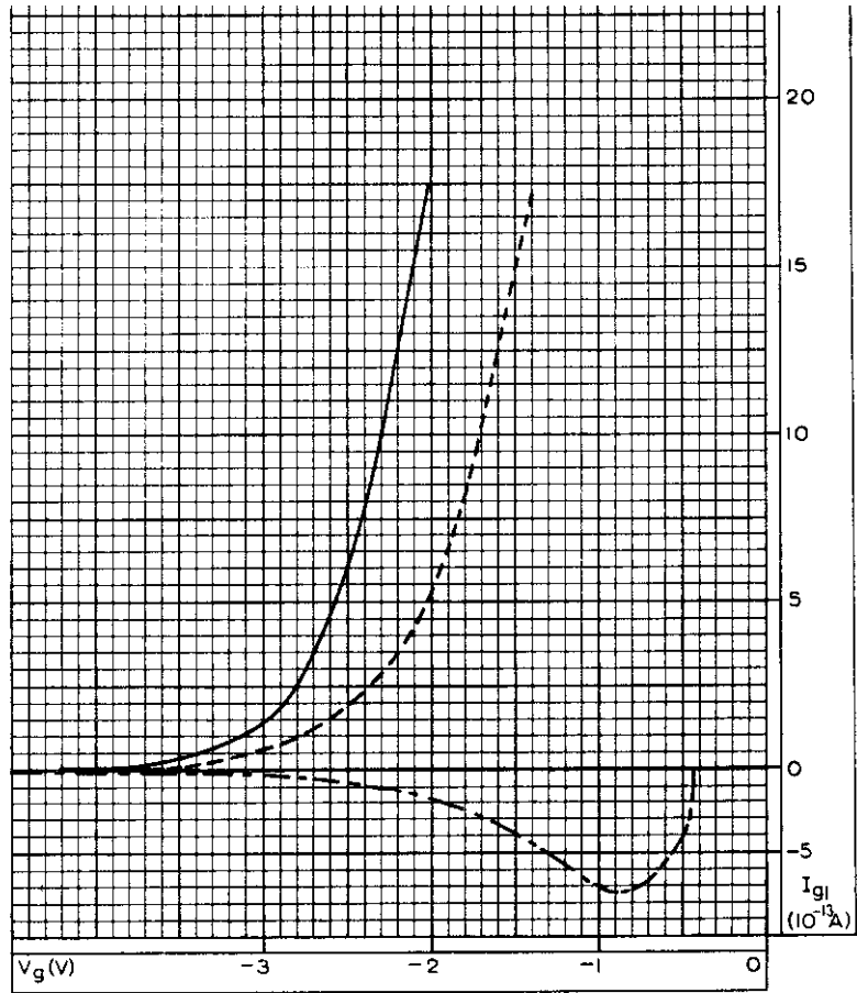
ANODE, SCREEN-GRID AND CONTROL-GRID CURRENTS PLOTTED AGAINST CONTROL-GRID VOLTAGE. V_a = 45V , V_{g2} = 6.5V
