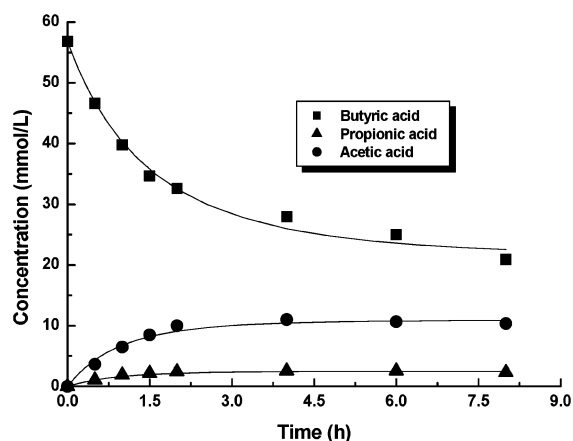
Figure 3. Comparison between the reaction–deactivation kinetic model proposed and the experimental results obtained in butyric acid oxidation with the Ir/C catalyst at 200 ^{\circ}\text{C} and 6.9 bar of oxygen partial pressure.
