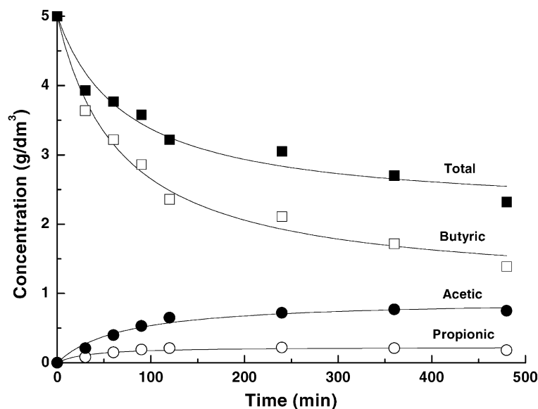
Fig. 2. Kinetics of BA ( 57 \text{ mmol dm}^{-3} aqueous solution) disappearance, and propionic and acetic acid formation, under the standard conditions ( 200^\circ\text{C} , 6.9 \text{ bar } P_{\text{O}_2} ).
