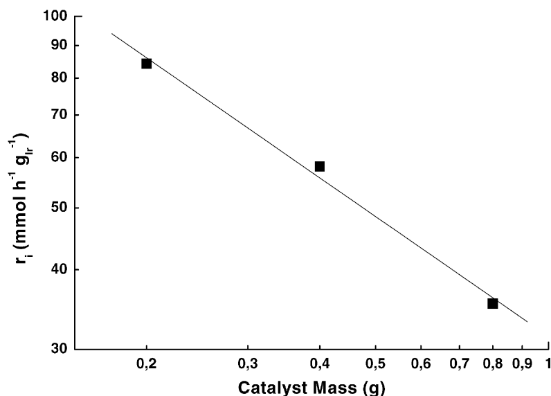
Fig. 3. Influence of the catalyst loading on the initial CWAO rate ( r_i , mmol h -1 g ir -1 ) of BA (57 mmol dm -3 ).
