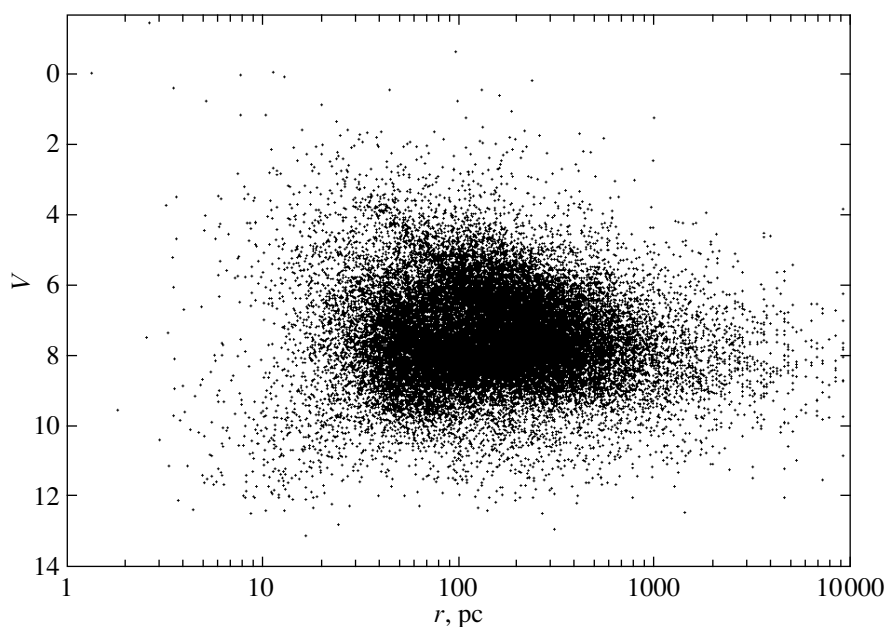
Fig. 7. Distribution of 35 495 PCR stars in distance and V magnitude.
