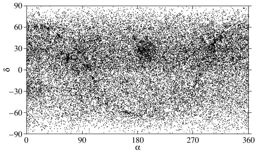
Fig. 5. Distribution of 35 495 PCR stars over the celestial sphere in equatorial coordinates.
