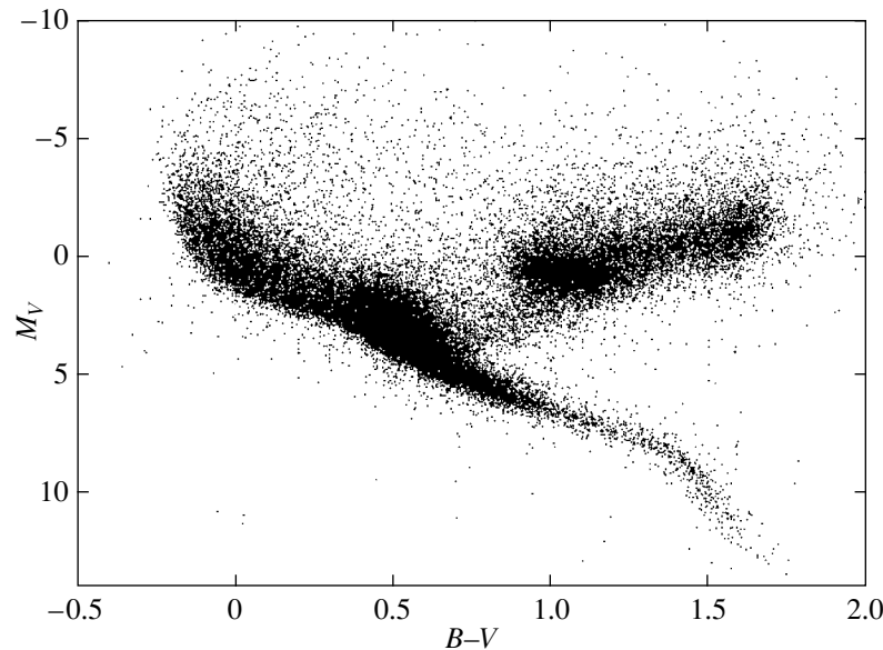
Fig. 6. Distribution of 35 495 PCR stars in B-V color index and absolute magnitude.
