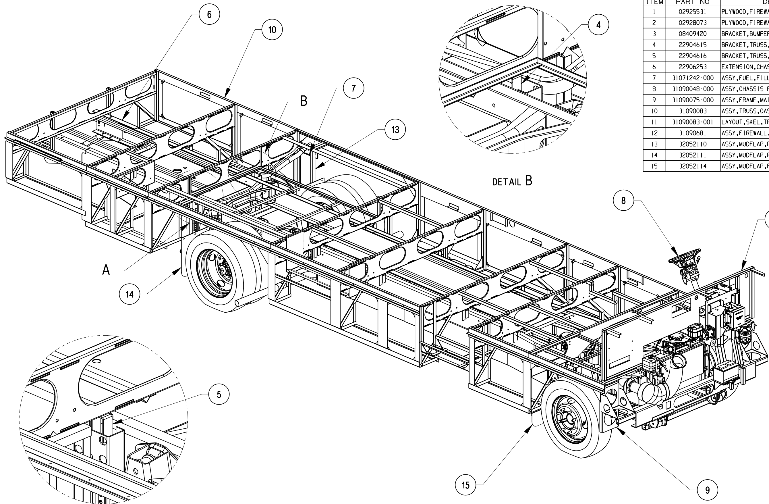
DETAIL A
