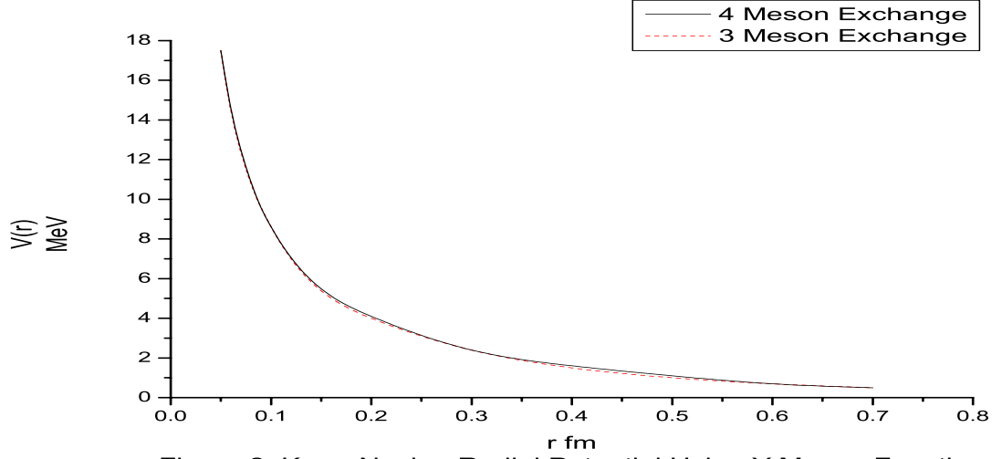
Figure 3: Kaon-Nuclon Radial Potential Using Y Meson Function
