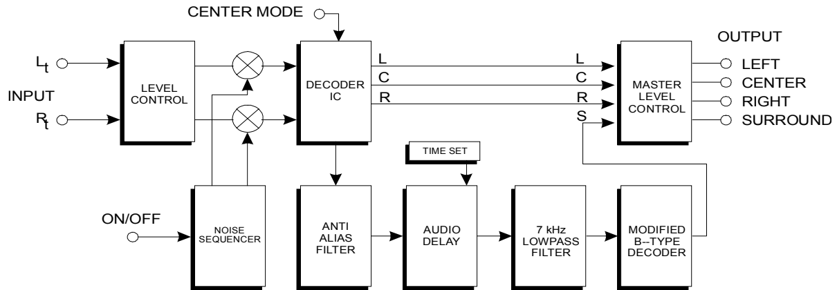
Figure 2-2 Dolby Surround Pro Logic Decoder
